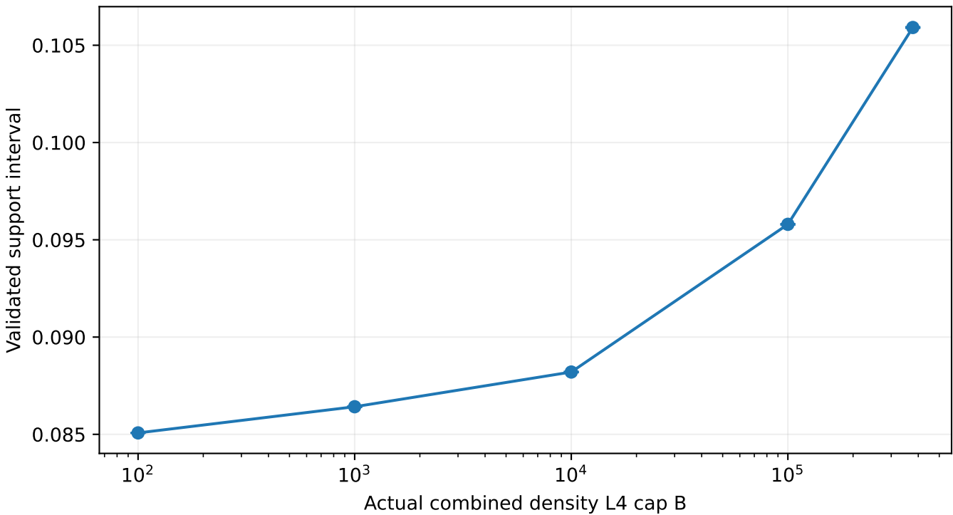
PV finite support: M=50 , L=10 , \epsilon=0.002
