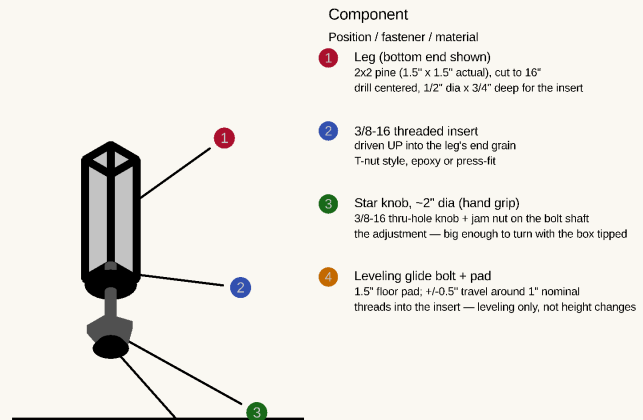
LEG LEVELING FOOT — shown 3x actual size (12 total: 4 per panel x 3 panels)
