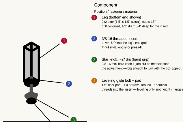
LEG LEVELING FOOT — shown 3x actual size (12 total: 4 per panel x 3 panels)
