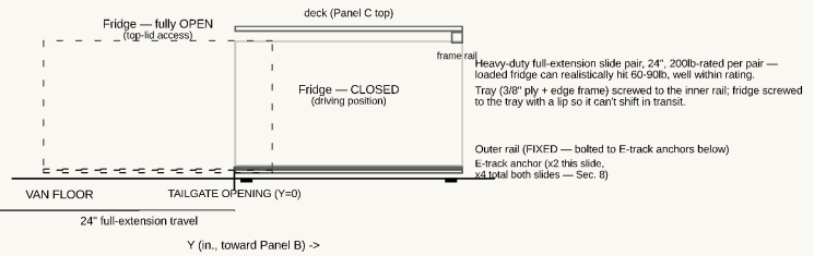
Fridge Slide Mechanism — side view (one of 2 parallel slides shown) CLOSED (solid) vs fully OPEN (dashed) — pulled out through the tailgate for top-lid access
