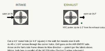
FAN MOUNTING — face-on, both fans identical hardware
