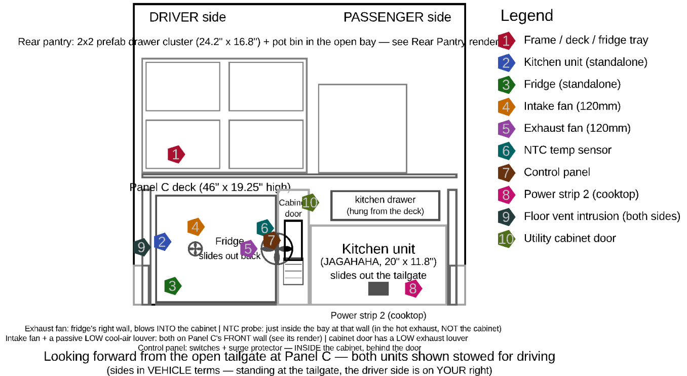
Rear view
