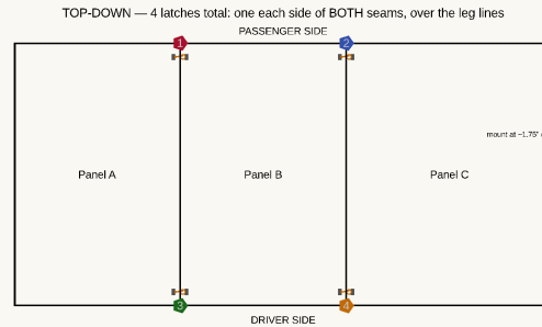
SEAM DRAW-LATCHES — clamp the 3 lift-out modules into one rigid beam (4 latches: both sides of the A/B and B/C seams) Alignment pins LOCATE the modules; the draw latches PULL them tight against the bumper. Hand-released — modules still lift out in seconds.
