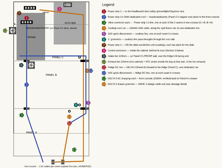
ELECTRICAL LAYOUT — top-down (front of van at bottom, tailgate at top)
