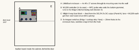
CONTROL CLUSTER — inside the cabinet on its backer board, elevation (looking forward from tailgate)
