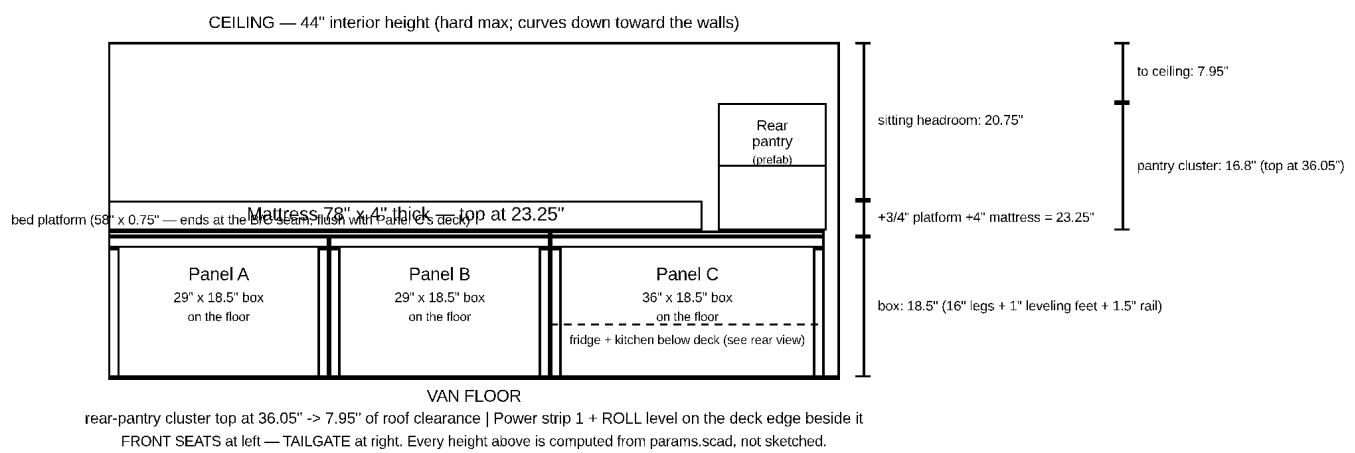
Side profile
