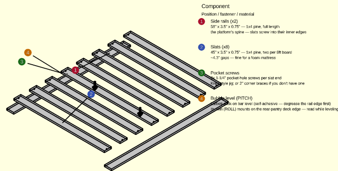
BED PLATFORM — flush ladder, exploded (Component 2, 58" x 52", 8 slats, 0.75" thick total) One 3/4" plane: slats sit BETWEEN the two full-length side rails, pocket-screwed — no battens below, nothing above. Rests DIRECTLY on Panel A/B's top rails and ENDS at the B/C seam, flush with Panel C's deck (the mattress's last ~20" rides that deck).
