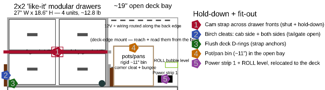
Panel C deck (46" wide, tailgate end) — cluster + bay just SIT on it, held by cleats + a strap
