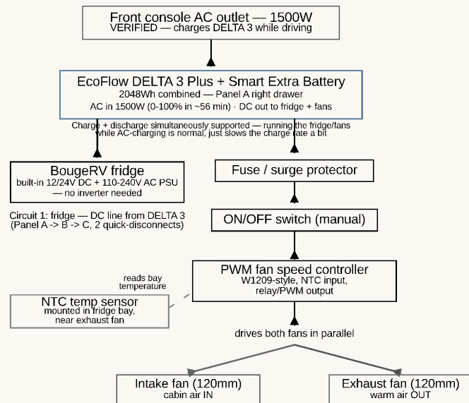
Fridge System Wiring — schematic, not to physical scale
