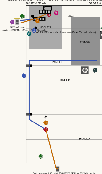
ELECTRICAL LAYOUT — top-down (front of van at bottom, tailgate at top)
