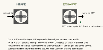
FAN MOUNTING — face-on, both fans identical hardware
