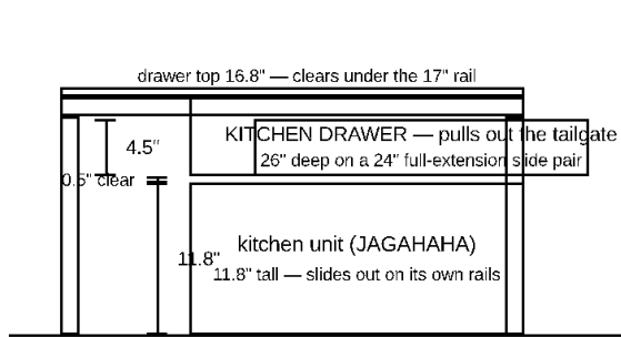
SIDE SECTION — front (B/C seam) at left, TAILGATE at right
