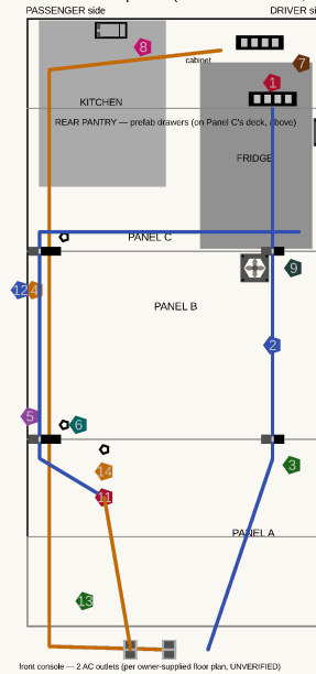
ELECTRICAL LAYOUT — top-down (front of van at bottom, tailgate at top)
