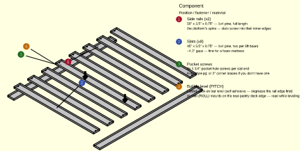
BED PLATFORM — flush ladder, exploded (Component 2, 58" x 52", 8 slats, 0.75" thick total) Rest DIRECTLY on Panel A's top rails and ENDS at the B/C seam. Flush with Panel C's deck (the mattress's last ~20" rides that deck).
