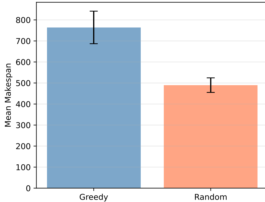
Makespan Comparison
