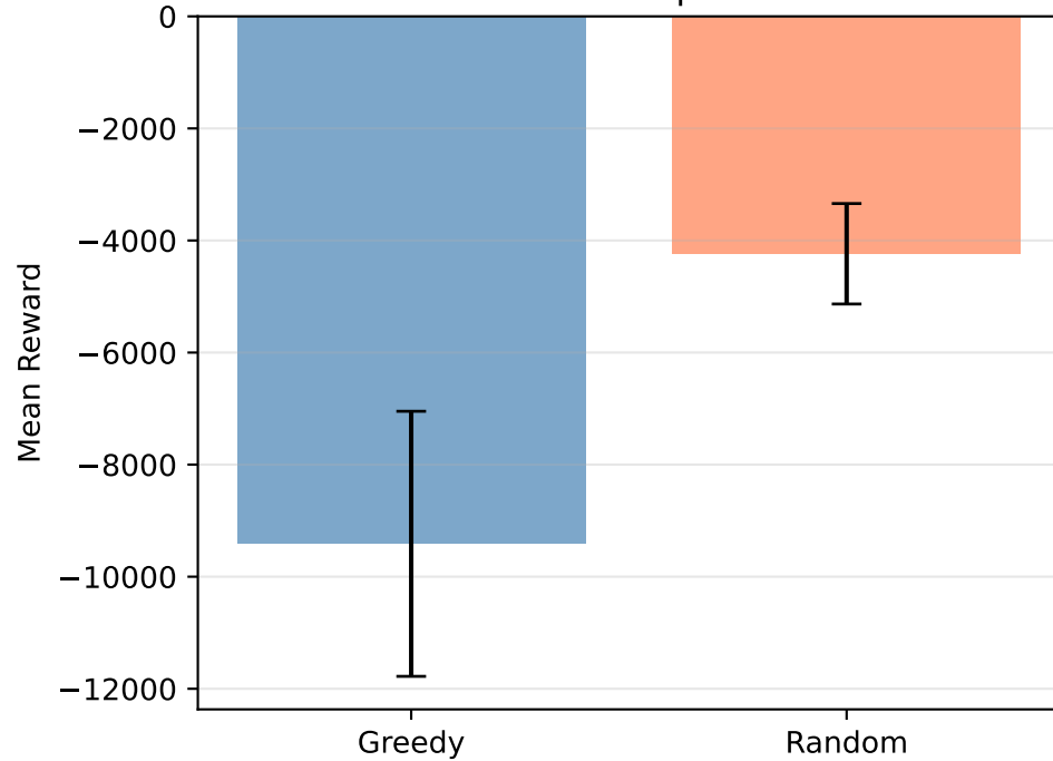
Reward Comparison
