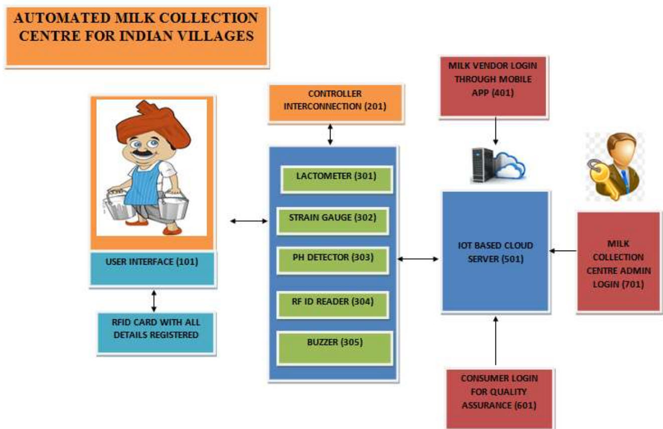
FIGURE 2: BLOCK DIAGRAM OF THE AUTOMATED MILK COLLECTION CENTRE FOR INDIAN VILLAGES
