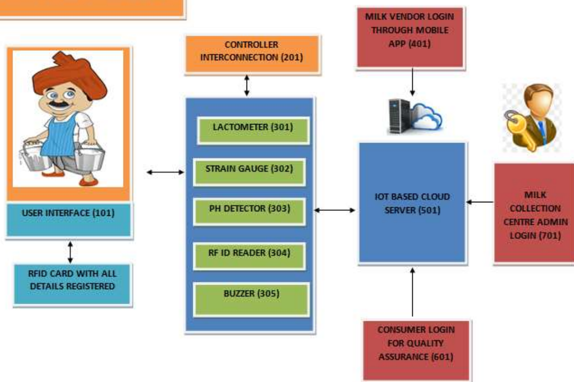
FIGURE 2: BLOCK DIAGRAM OF THE AUTOMATED MILK COLLECTION CENTRE FOR INDIAN VILLAGES
