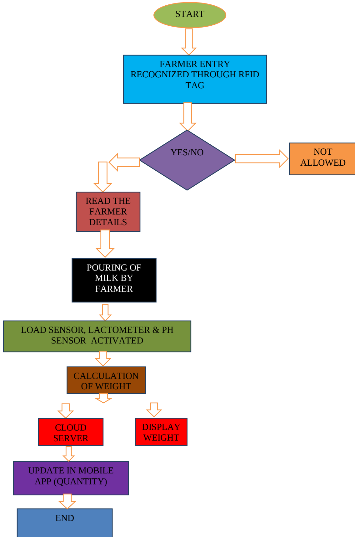
FIGURE 1: FLOW CHART OF THE AUTOMATED MILK COLLECTION CENTRE FOR INDIAN VILLAGES
