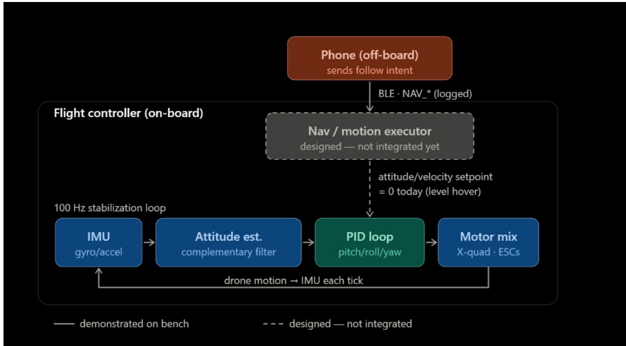
Figure 1: Two-layer flight control loop
