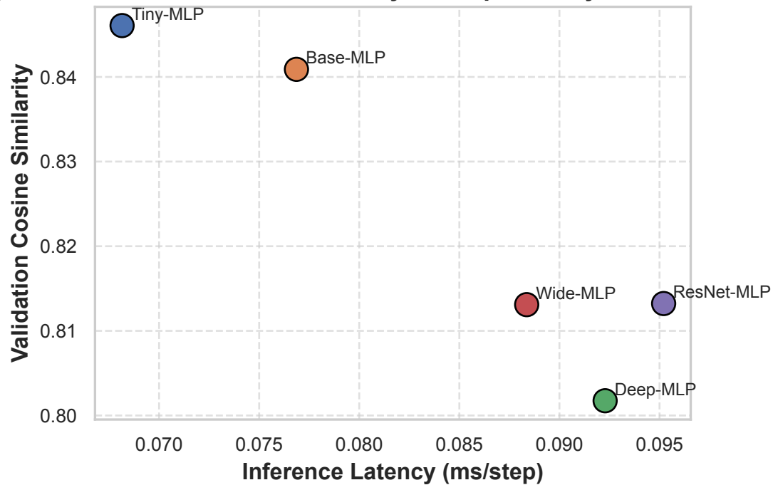
Distillation Quality vs Step Latency
