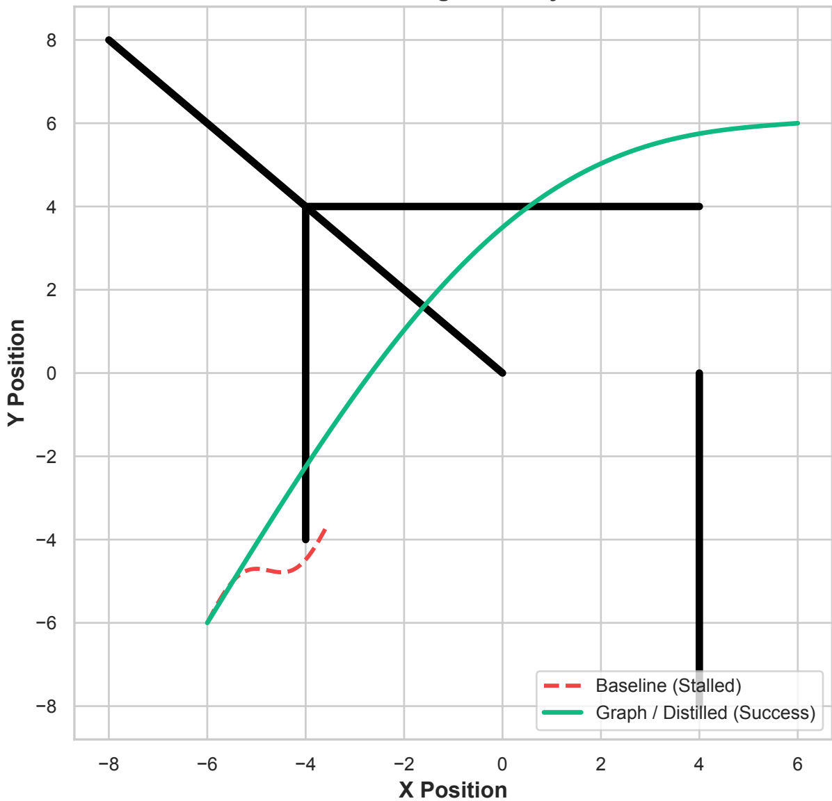
Qualitative Navigation Trajectories
