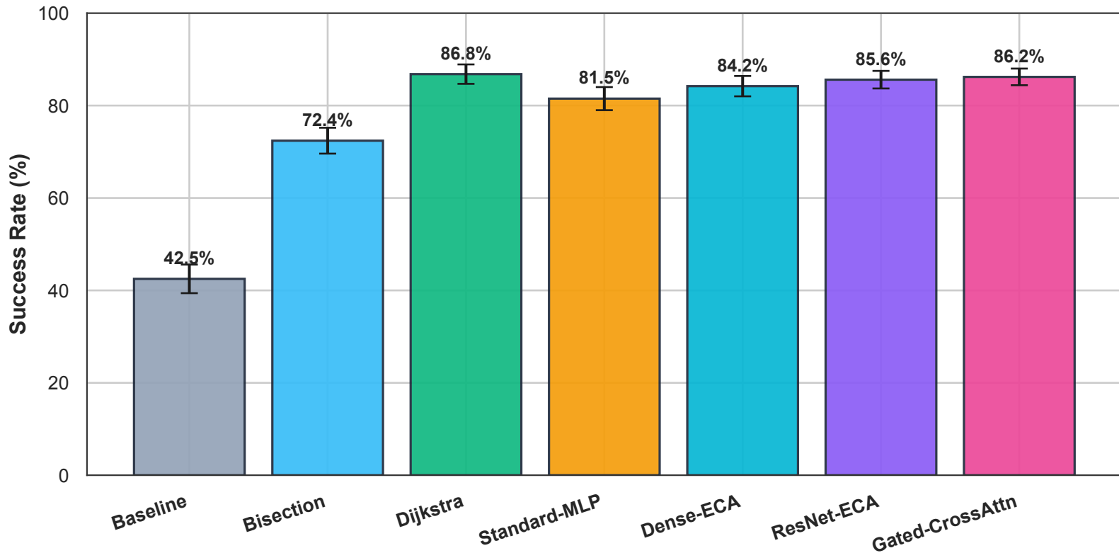
Navigation Success Rate on antmaze-medium-navigate-v0 (10 Seeds)
