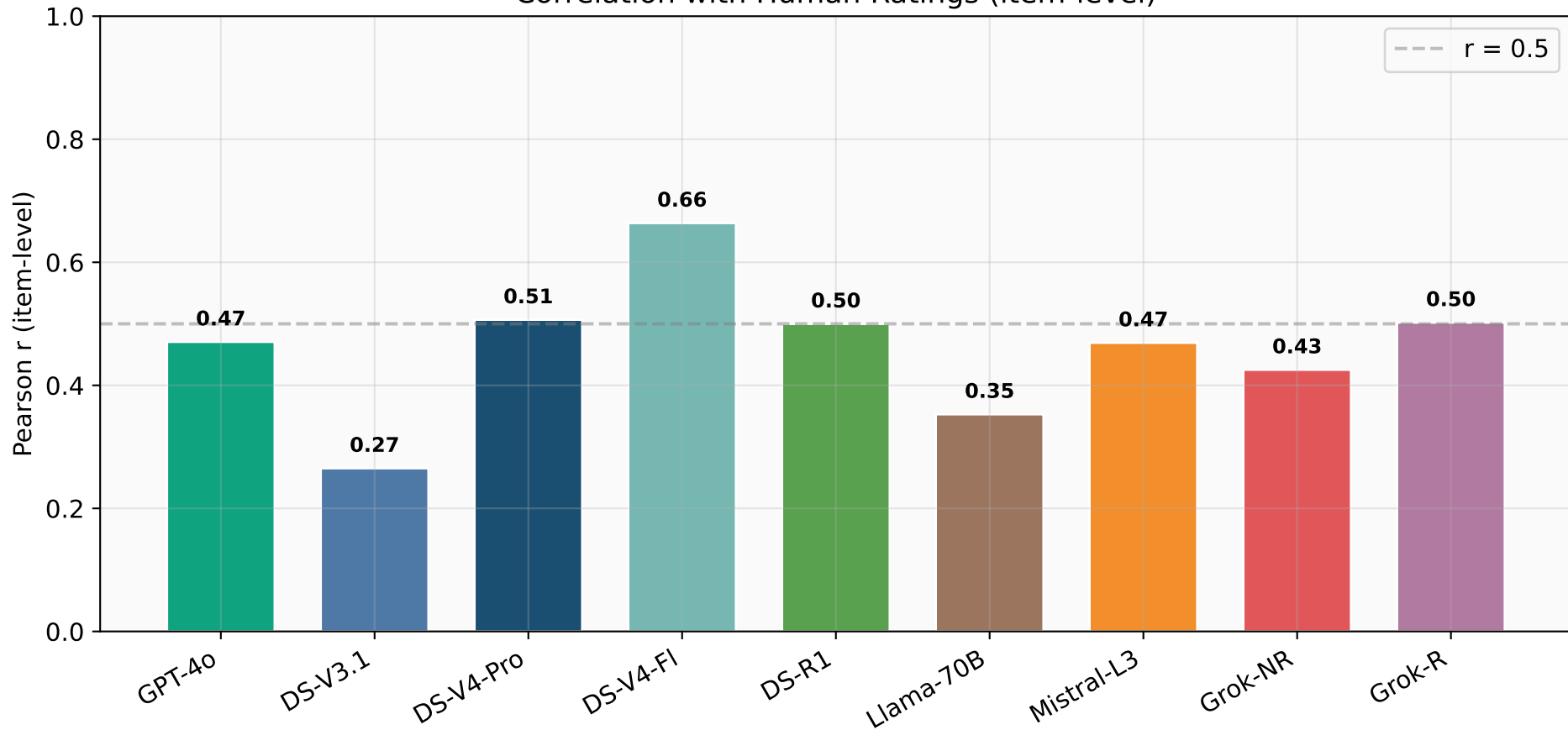
Correlation with Human Ratings (item-level)
