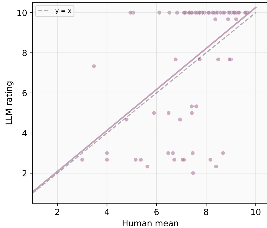
Grok-R (r=0.50)
