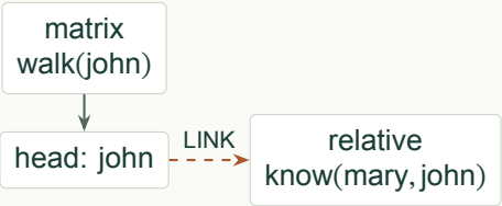
Schematic: functor branches and intermediate states omitted.
