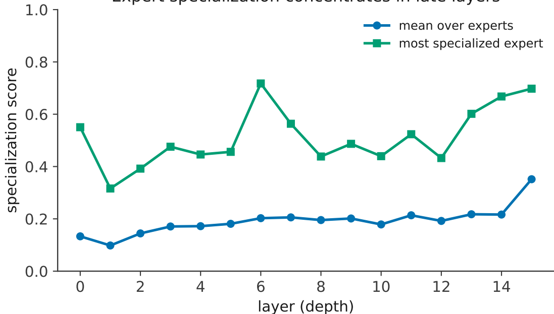
Expert specialization concentrates in late layers
