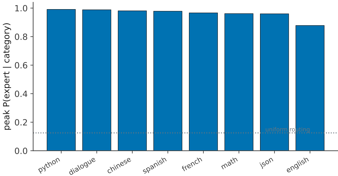
Every category has a strongly dedicated expert
