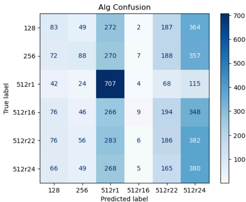
Fig 16: Confusion Matrix of Attempted Classification
