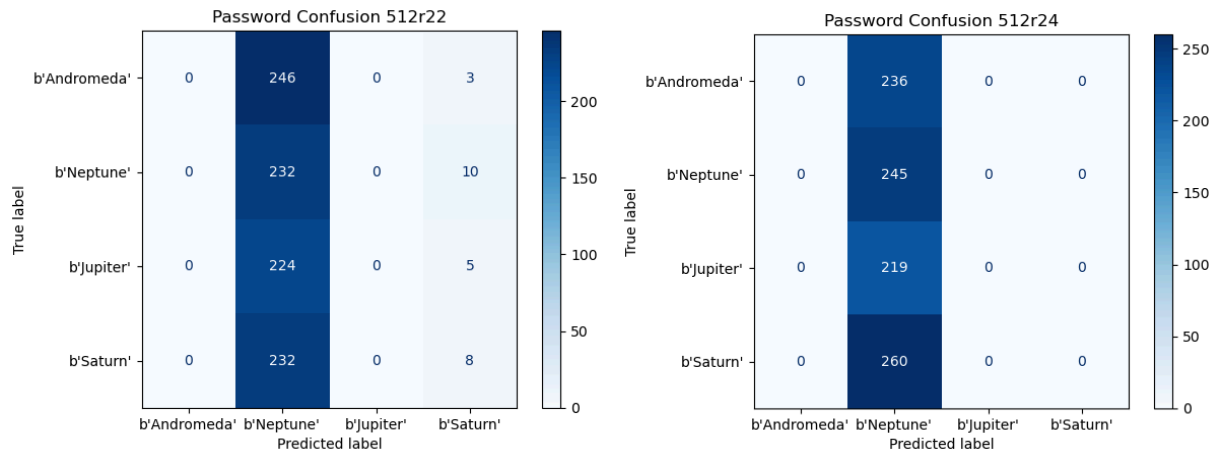
Fig 17: Confusion Matrices of Password Classification
