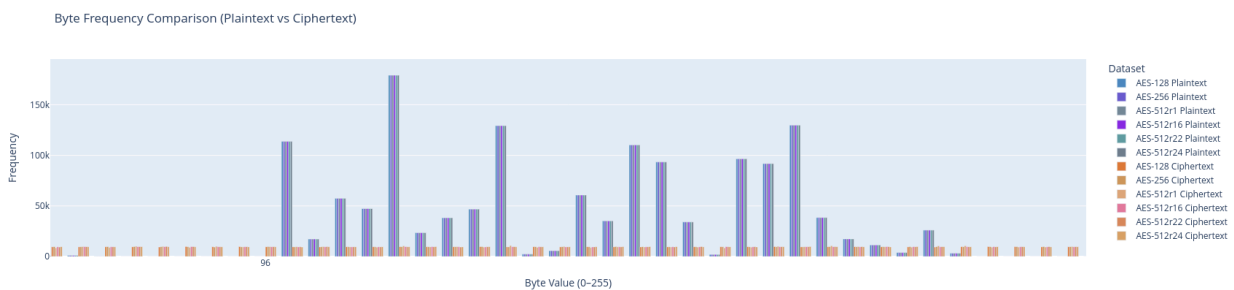
Fig. 18: Byte Frequency Histogram
