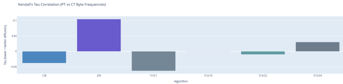
Fig. 20: Tau Correlation Plot
