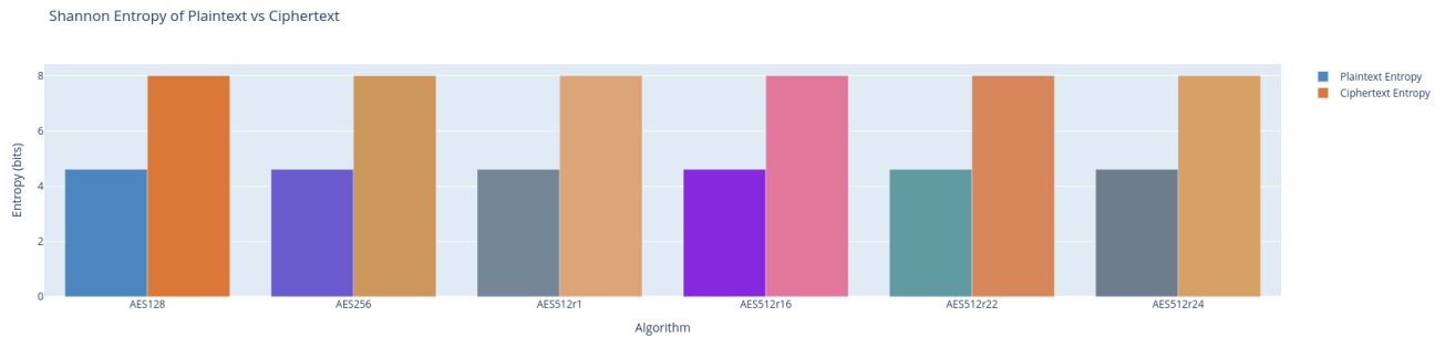
Fig. 19: Shannon Entropy of Plaintext and Ciphertext
