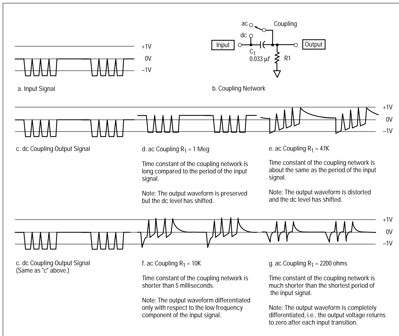
Figure 9. dc and ac Coupling for a complex pulse train.
