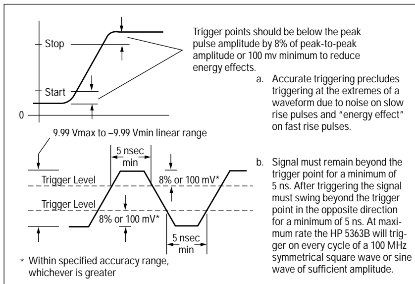
Figure 38. Input Signal requirements for the HP 5363B.
