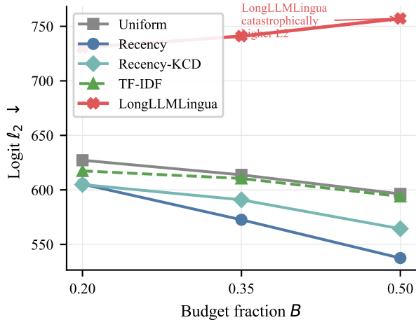
(a) External baselines ( n = 1,000 conv)
