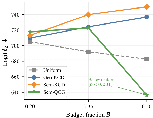
(b) KCD signal variants ( n = 50 conv)
