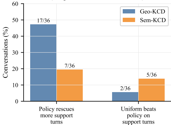
(a) Support-turn rescue rate (budget B = 0.35 , n = 36 conv)
