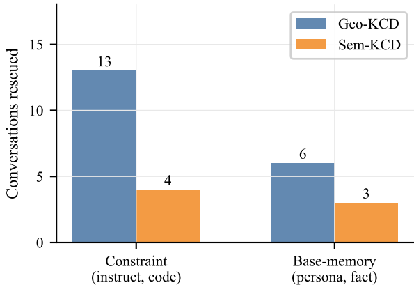
(b) Rescue breakdown by turn family
