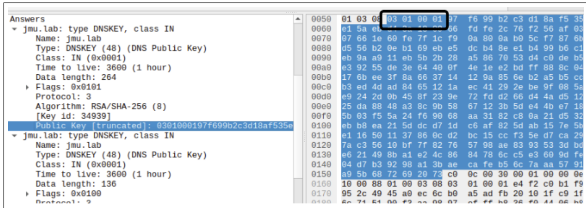
Figure 5.16: Wireshark traffic showing the first four bytes of the public key material, followed by the rest of the key.
