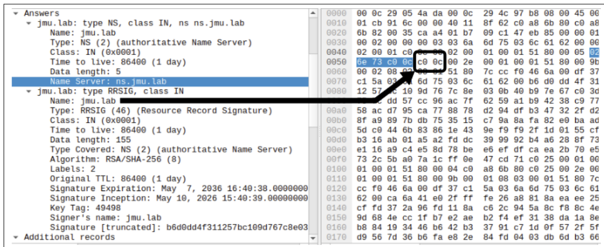
Figure 5.11: A screenshot of Wireshark showing a compressed name, as well as other data in order. You can see in the blue highlighted area is the name server's name, with the uncompressed ns and the compressed pointer for the rest of the name.
