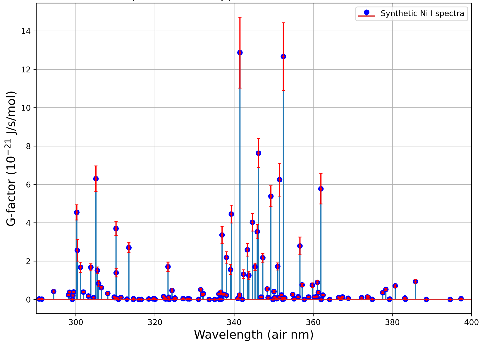
Ni I Fluorescence Spectrum with approximate errorbars based on 100 iterations
