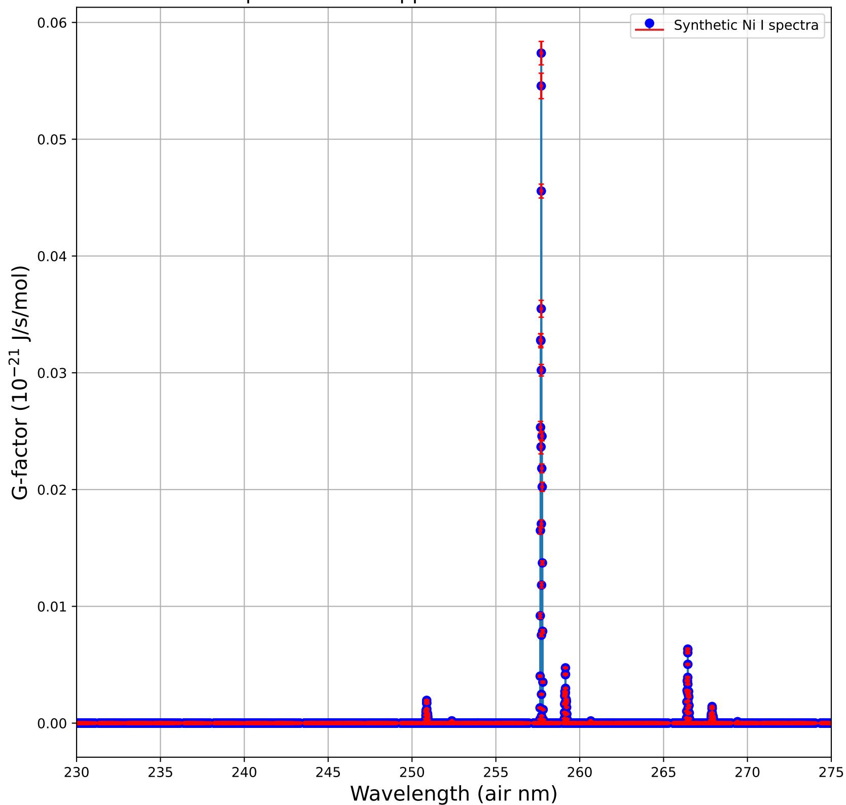
CS Fluorescence Spectrum with approximate errorbars based on 10 iterations
