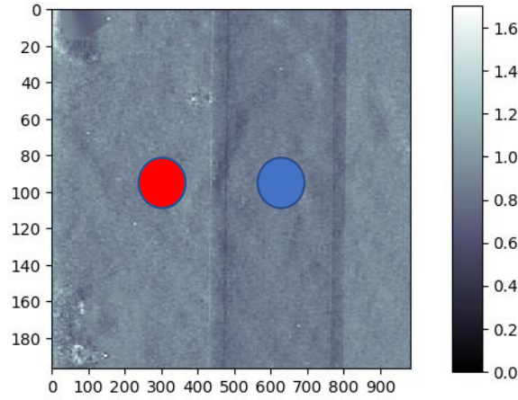
Figure S2. Visualization of the regions selected in the CI_- image at the energy-bin 13–16 keV for evaluating the \Upsilon matrix and the \zeta function.
