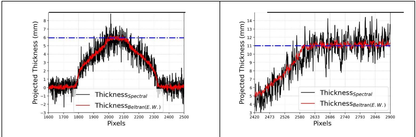
Figure S6. Comparison of the retrieved projected thickness profiles of bone and air, obtained using the spectral multi-material decomposition approach and the energy-weighted Beltran approach, with the theoretical projected thicknesses in the selected regions.
