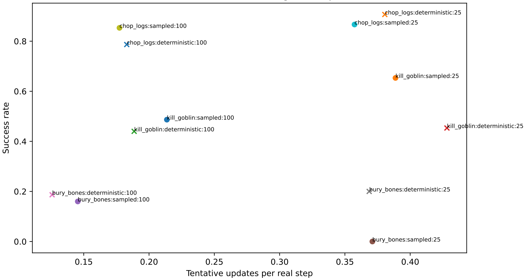
Performance versus virtual-gate compute
