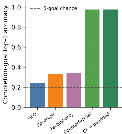
Goal identification
