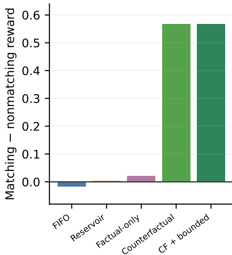
Reward selectivity
