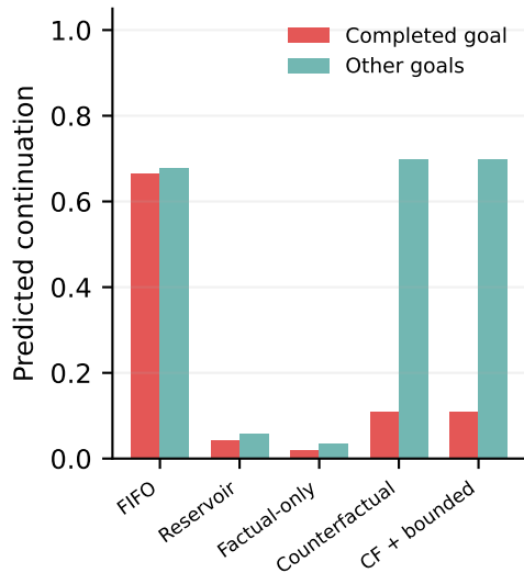
Goal-specific stopping
