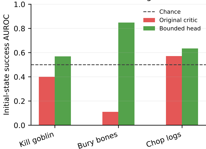
Success ranking
