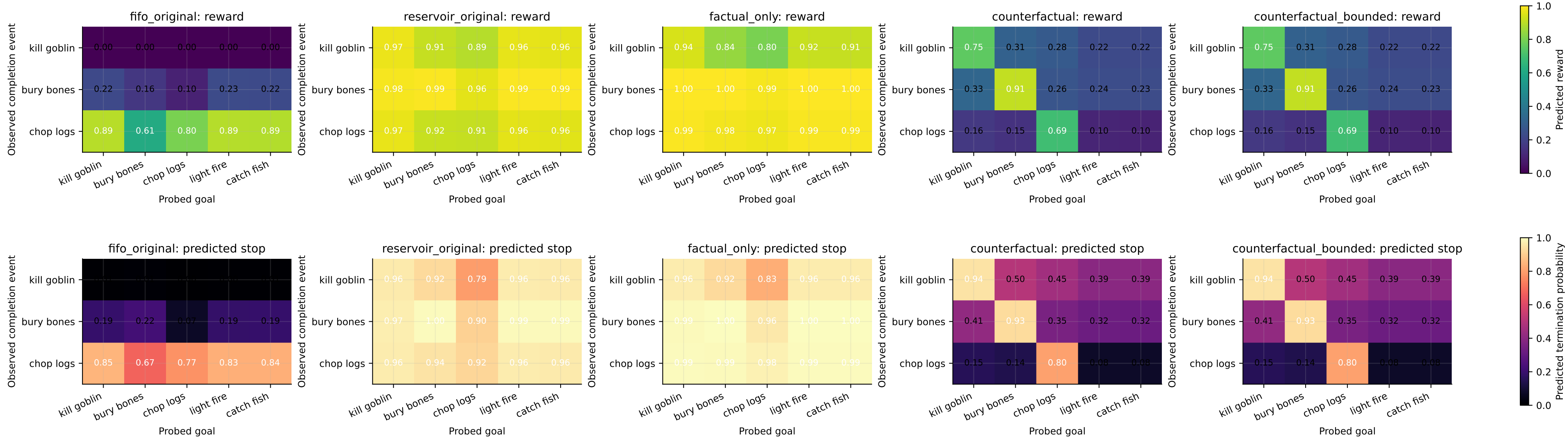
Goal-conditioning confusion on genuine completion states
