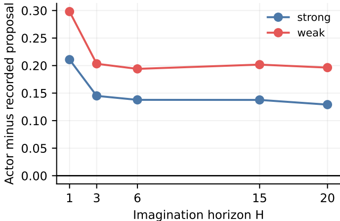
Bootstrap difference
