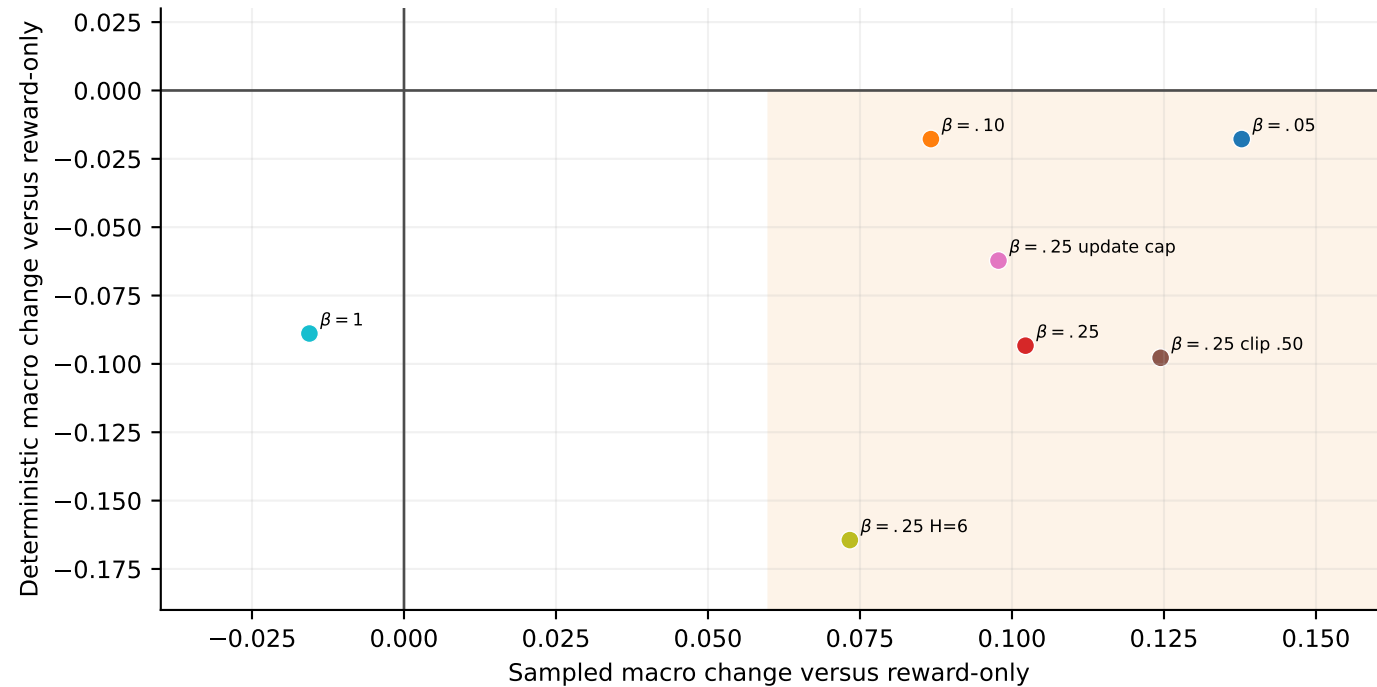
Small value doses improve sampling without improving the mode
