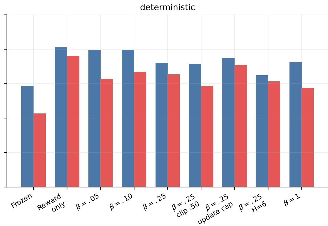
Stage 4B mean and worst-goal safety
