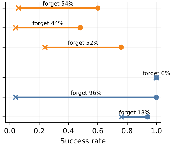
Deterministic policy
