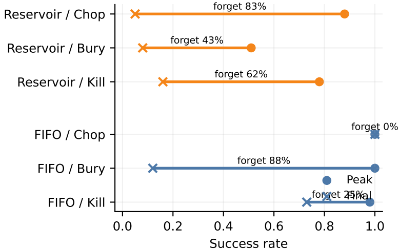
Sampled policy
