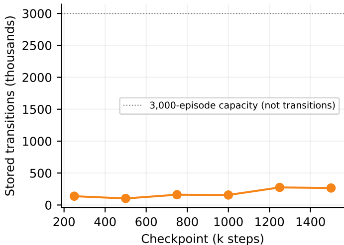
Variable-length reservoir occupancy
