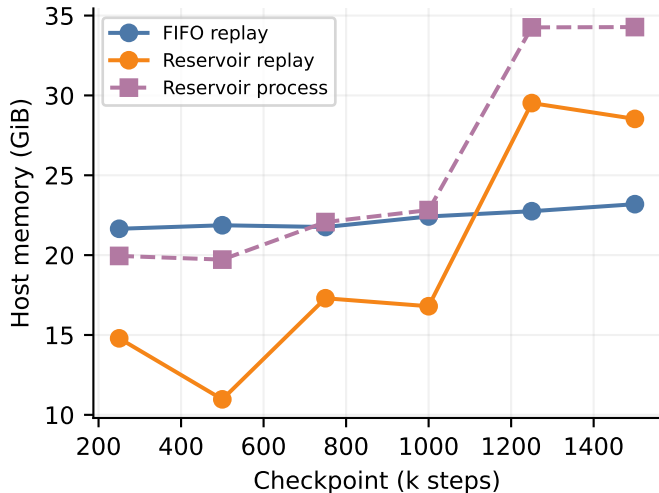
Host-memory footprint
