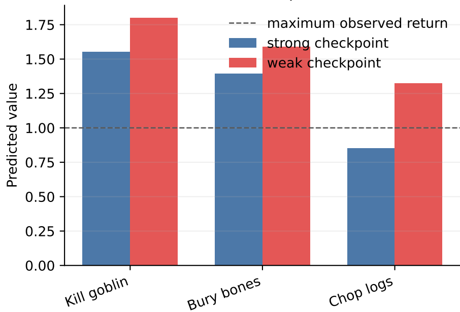
Critic on identical episode starts
