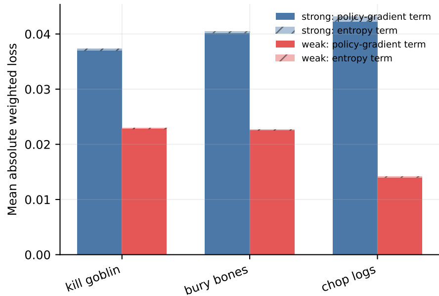
Actor-loss magnitude decomposition
