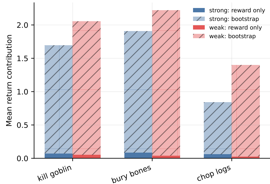
Lambda-return decomposition
