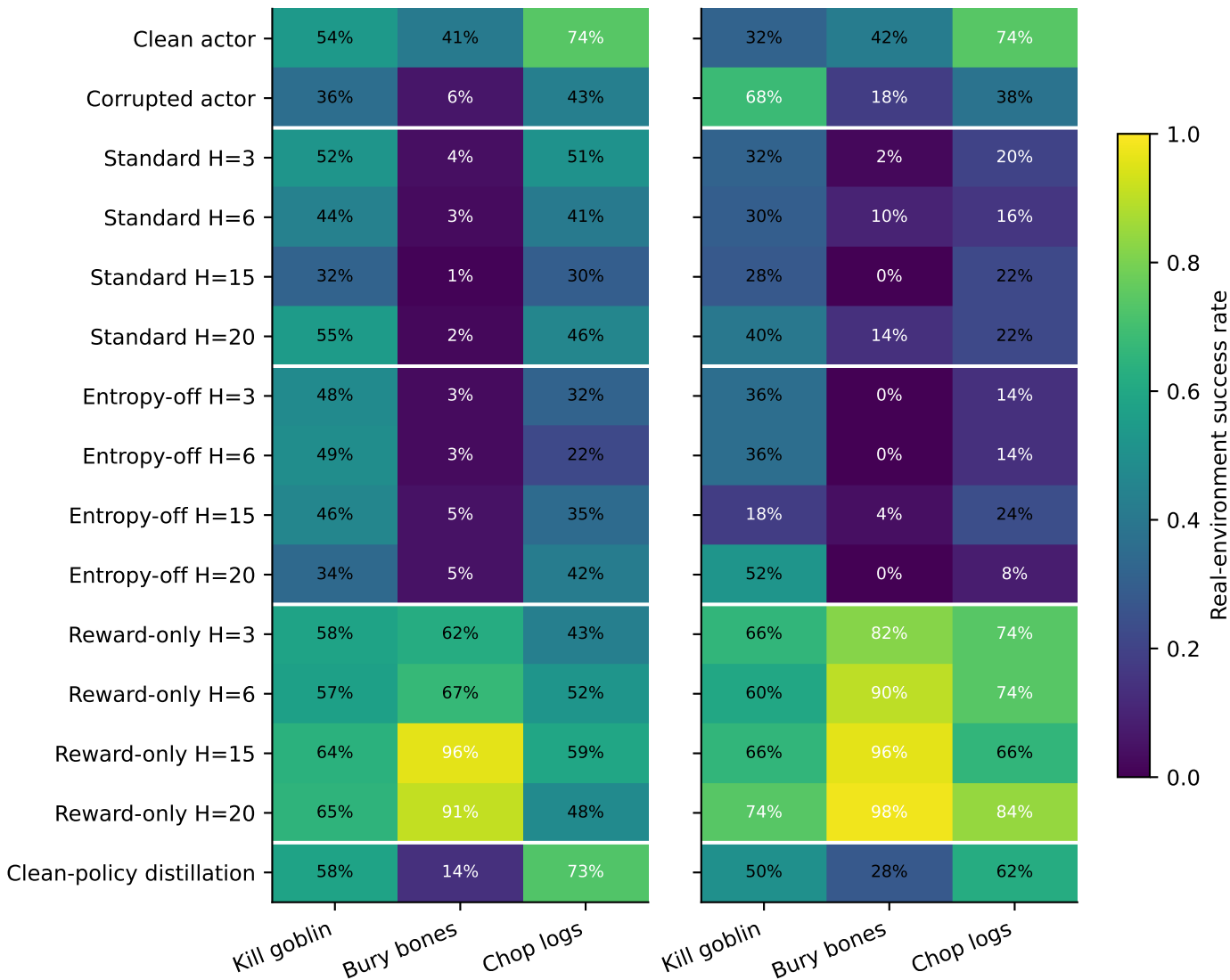
Sampled policy
