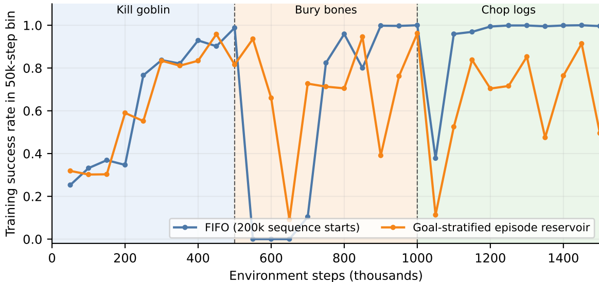
Sequential task acquisition is strong but reservoir training is less stable
