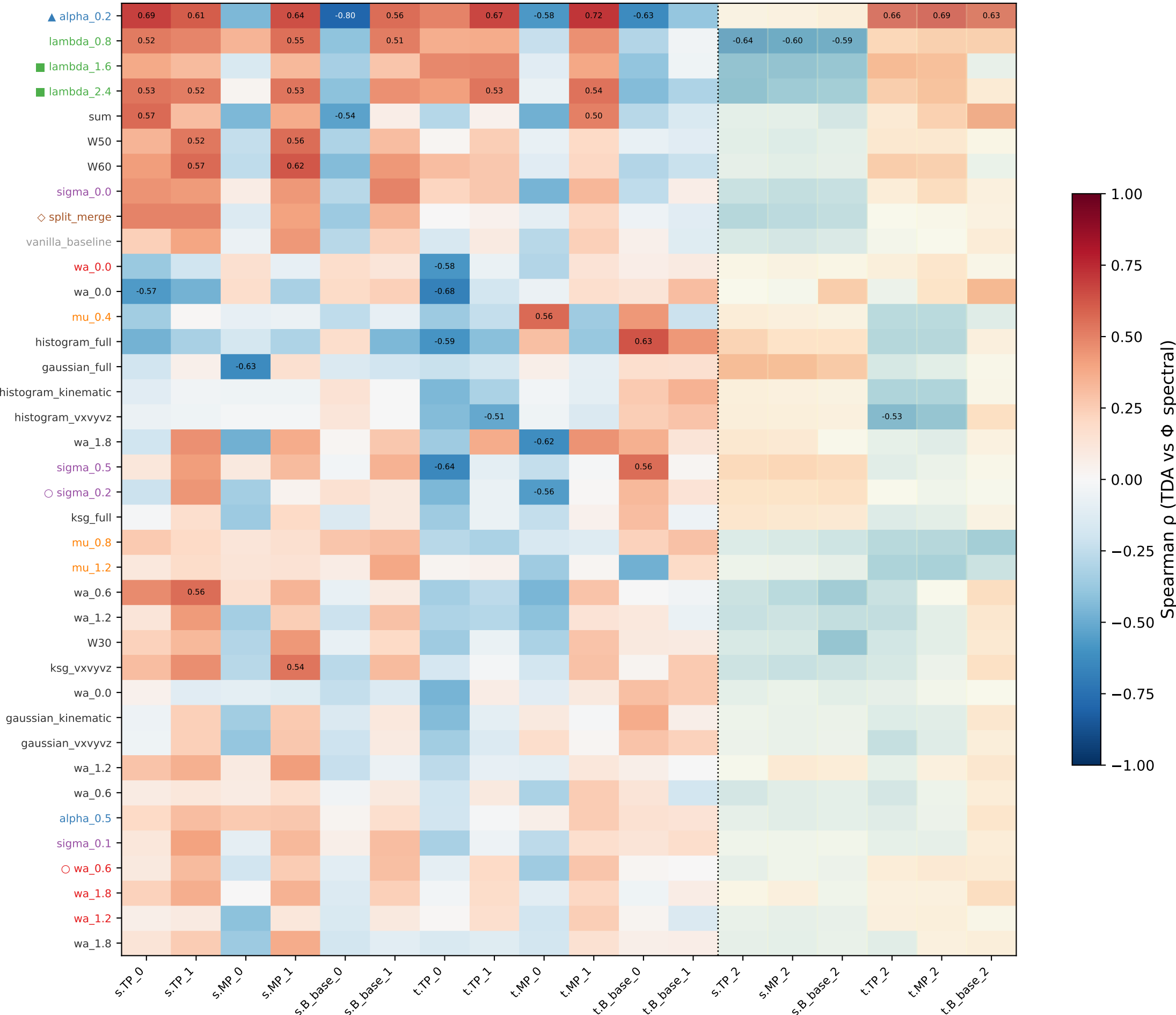
Agreement/Divergence: Spearman \rho between \Phi spectral and 18 TDA metrics (38 scenarios, hierarchical row clustering; H2 columns shaded; ○=$4.2 ▲=$4.3 ■=leader-block ◇=exploratory)
