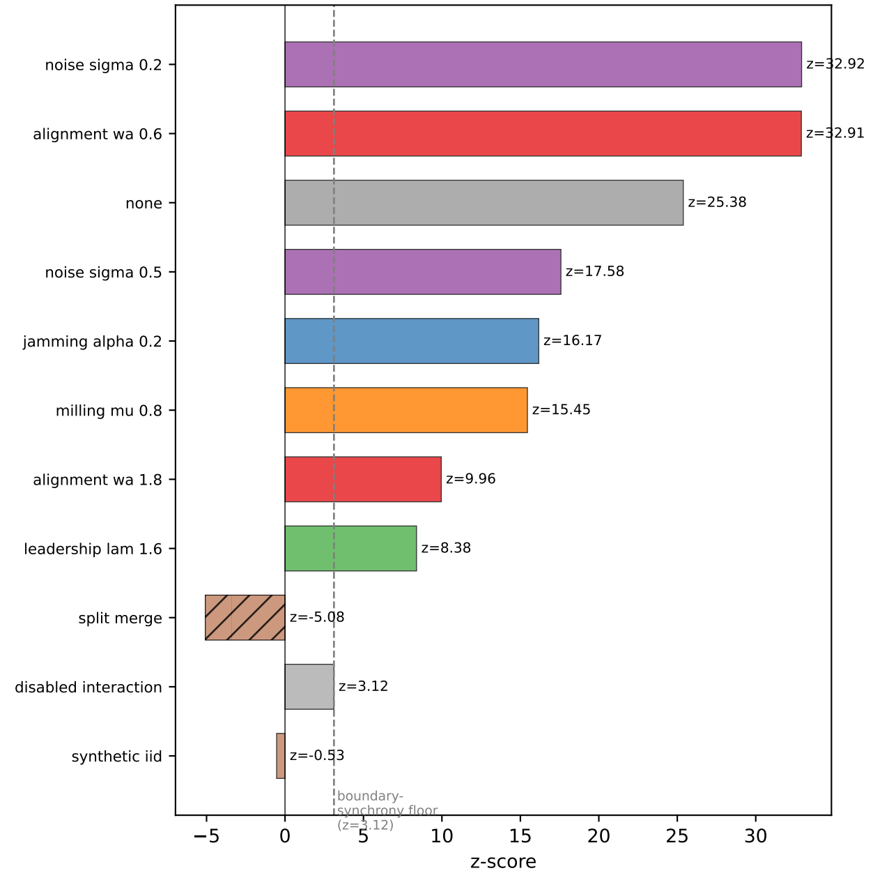
Surrogate z-scores (dashed = boundary-synchrony floor z=3.12 )
