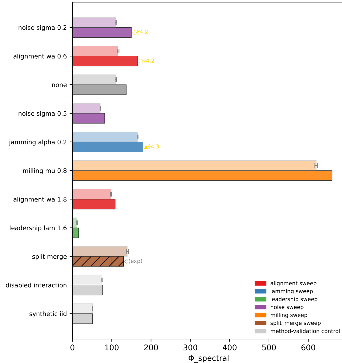
Observed vs surrogate \Phi (dark=observed, light=surrogate \pm 95% CI)
