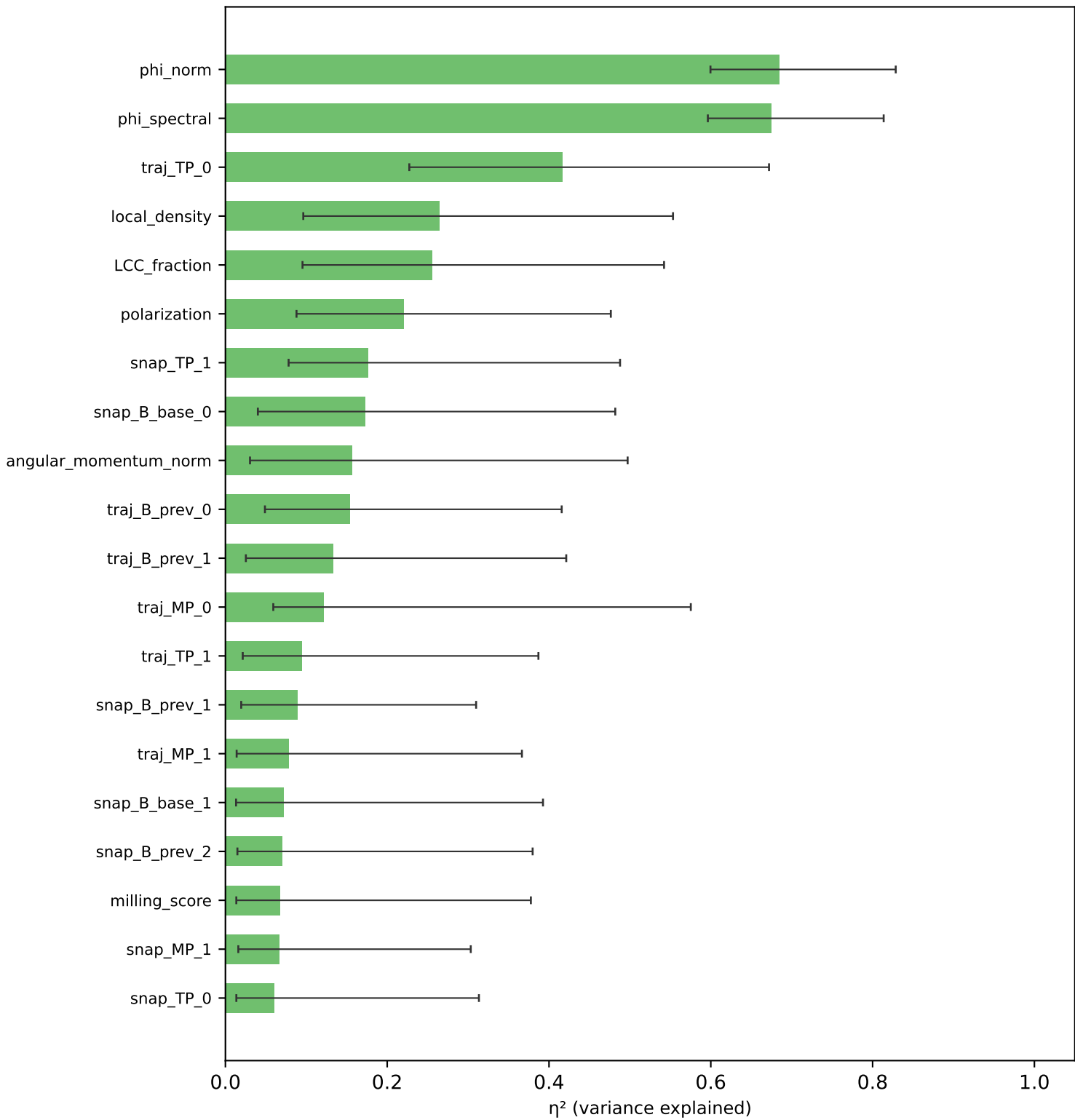
Sensitivity: leadership_sweep
