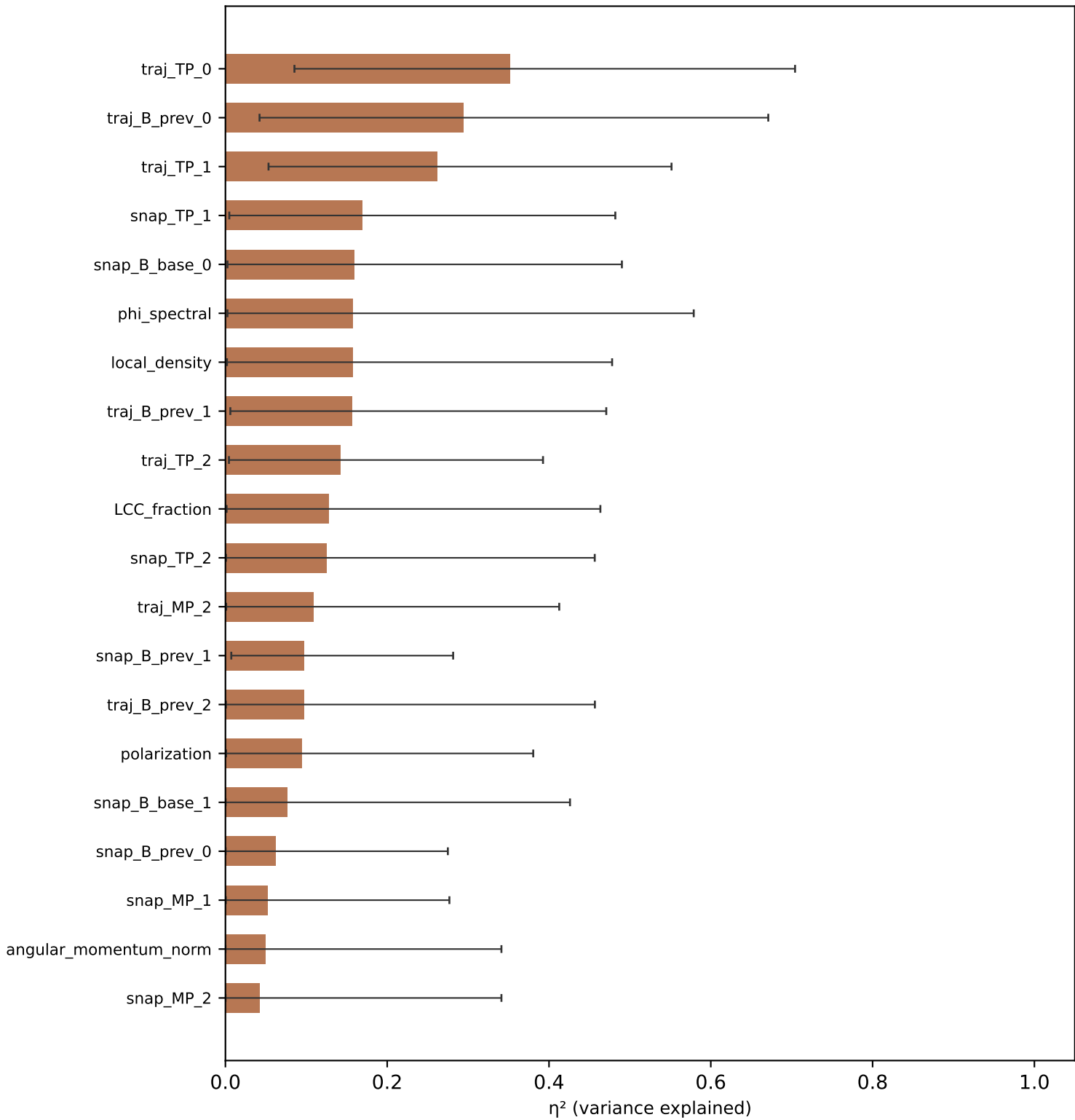
Sensitivity: split_merge_sweep
