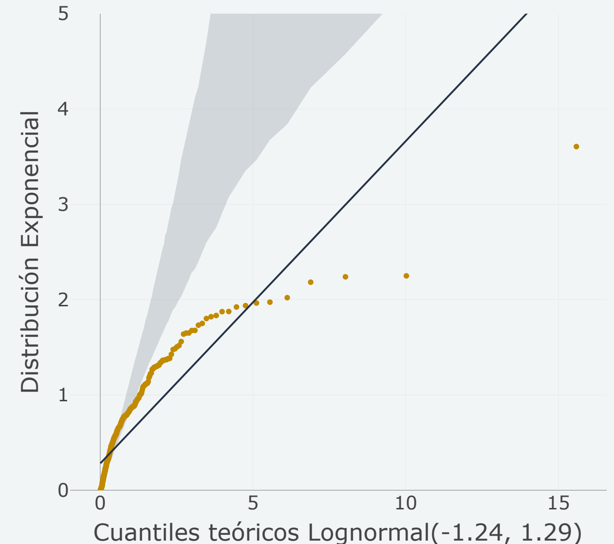
QQ-plot (lognormal)
